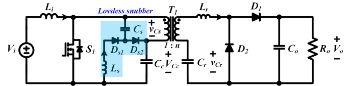
Fig. 1. Proposed isolated single switch ZCS–ZVS converter.
