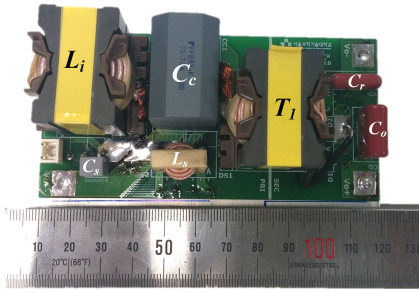
Fig. 15. Photograph of the proposed converter prototype.
